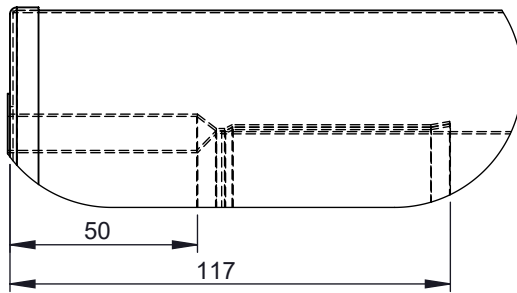
DETAIL A (1 : 2)
